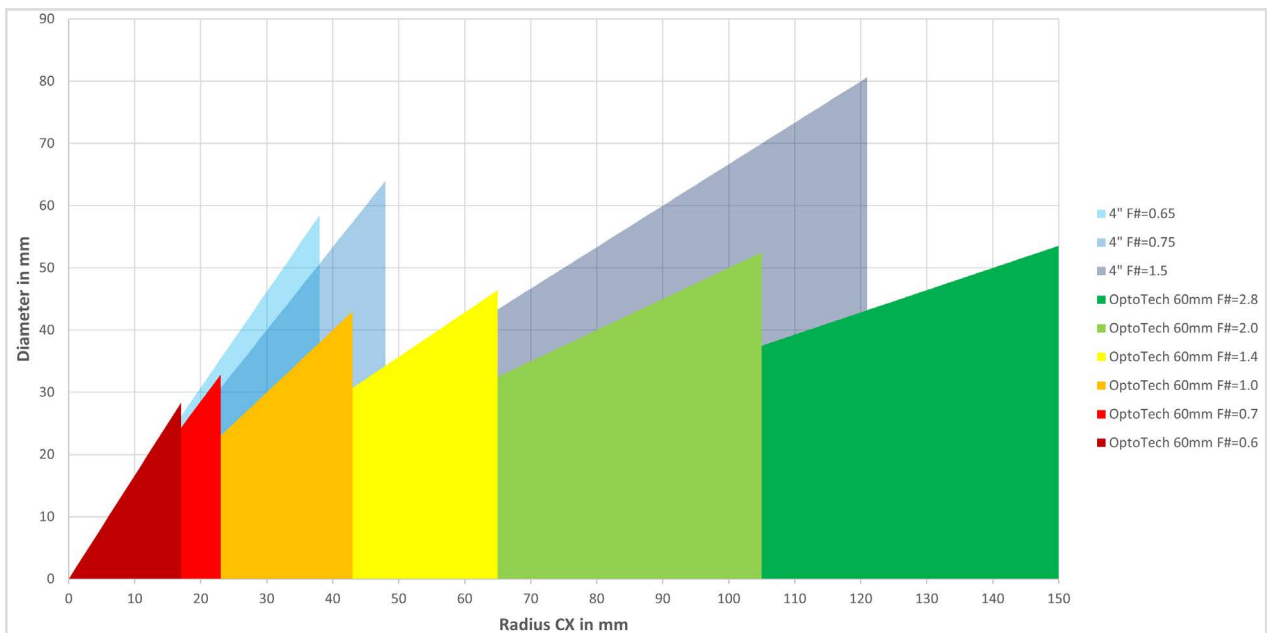
Comparison: Measuring range OptoTech 60mm reference spheres vs. measuring range 4" reference spheres
