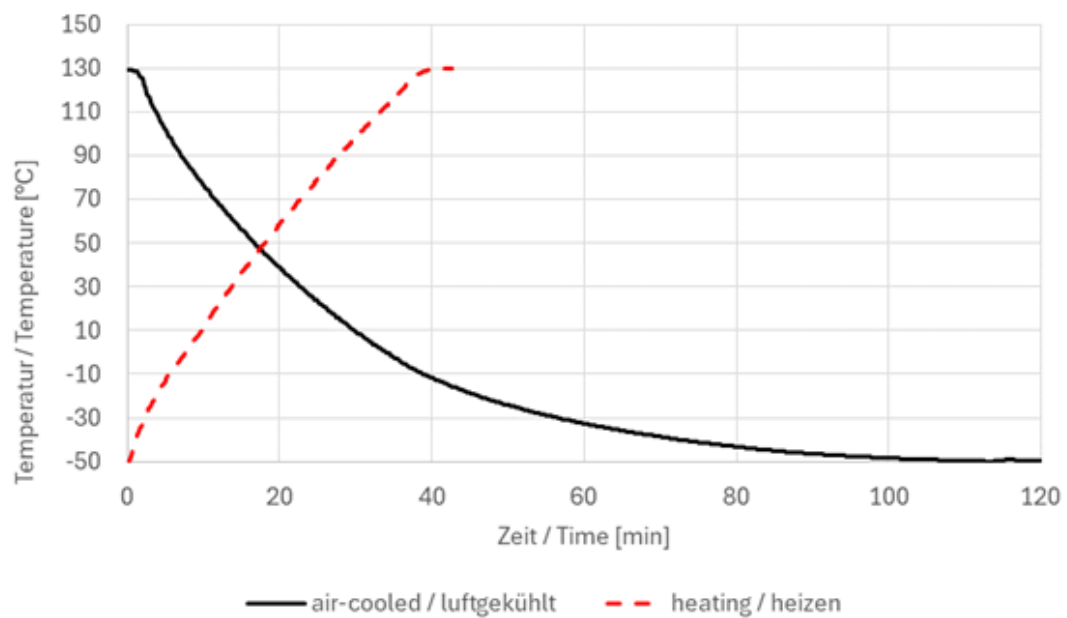
Cooling and heating curve LabEvent T/500/50/3
