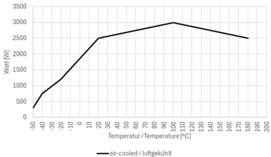
Heat compensation curve LabEvent T500/50/3
