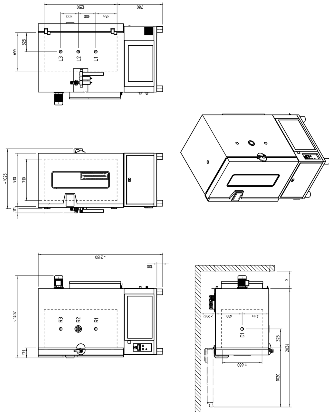
Installation drawing LabEvent T/500/50/3
